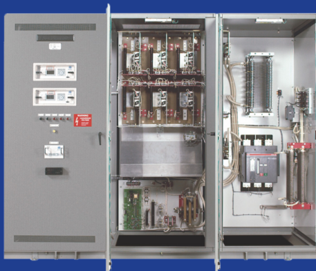
Dual channel DECS-400 controllers
